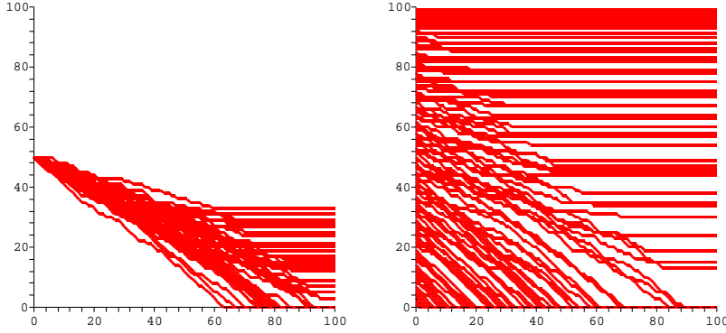
Figure 11: Left: Fifty random evolutions in the fair case m = n = 50 . Right: Random evolutions in the general case m + n = 100 , with m \in [1..99] . The horizontal axis represents time, the vertical axis corresponds to the size of the first group.
