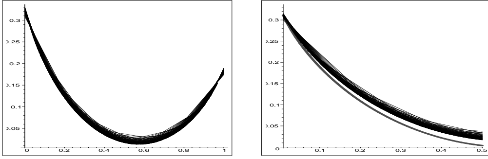
Figure 8: The 2–3 tree urn model. Left: a plot of \{-\frac{1}{n} \log \mathbb{P}(A_n = k)\}_{k=0}^{n+1} against k/(n+1) , for n = 24 \dots 96 ; right: a comparison against the limit large deviation rate function.
